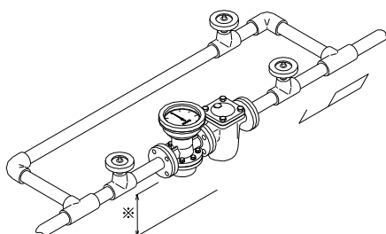
Horizontal piping (Horizontal installation)
