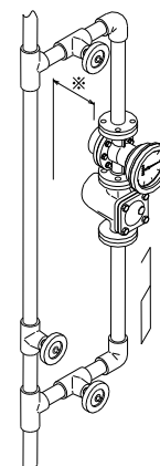
Vertical piping
